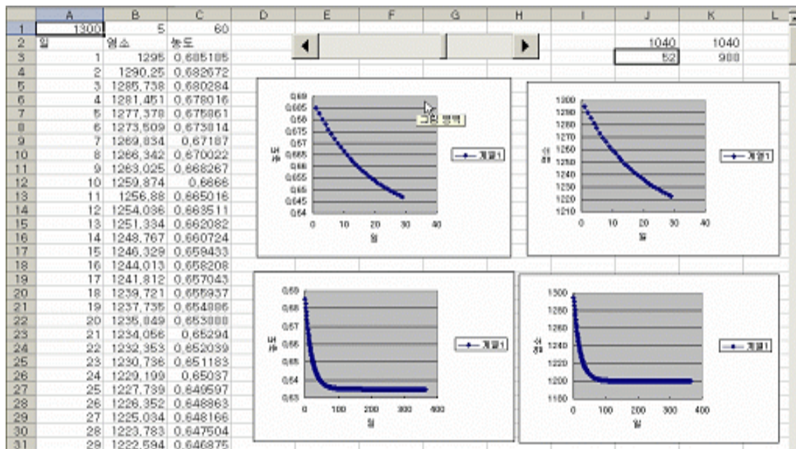
Figure 2: Changes in the concentration and amount of chlorine with initial amount 1040g (above) and 1300g (below)
